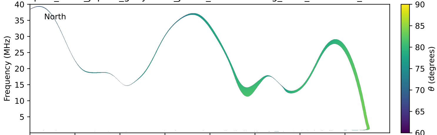
expres_earth_jupiter_ganymede_jrm33_lossc-wid1deg_3kev_20250618_v11.cdf
