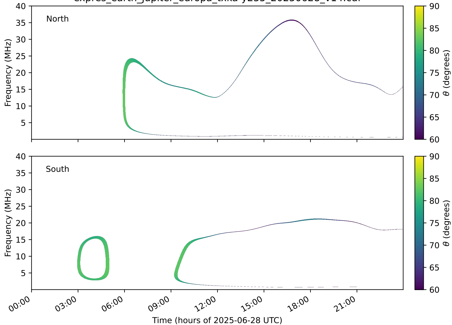
expres_earth_jupiter_europa_txka-y235_20250628_v14.cdf
