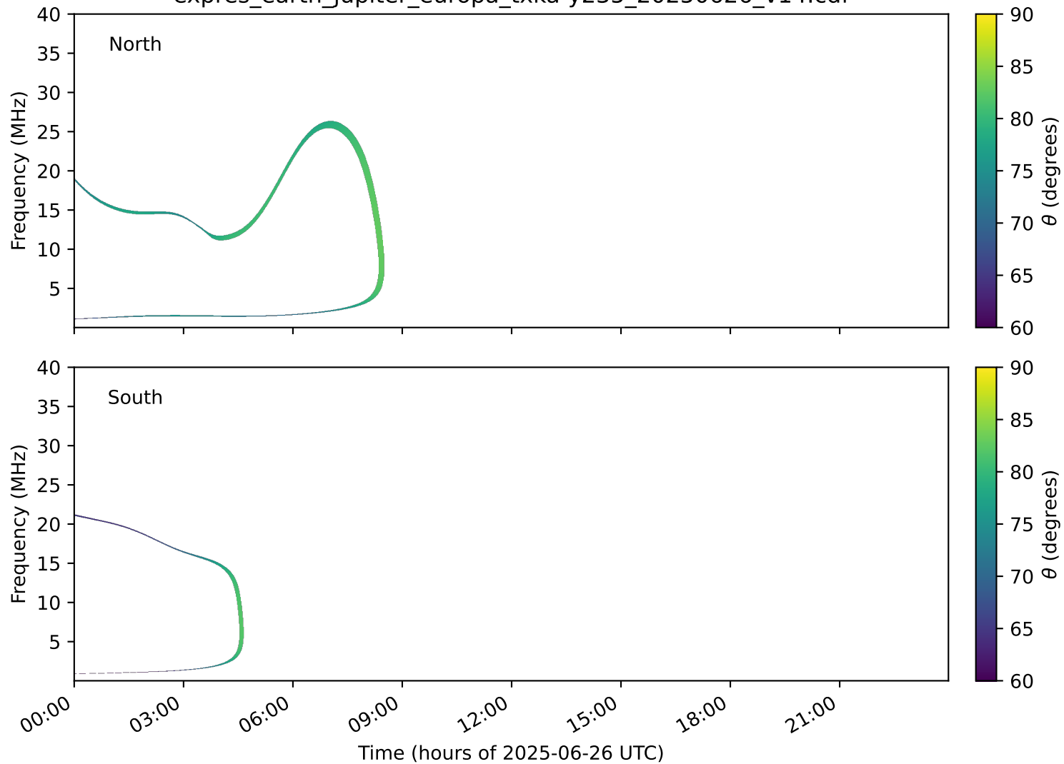
expres_earth_jupiter_europa_txka-y235_20250626_v14.cdf
