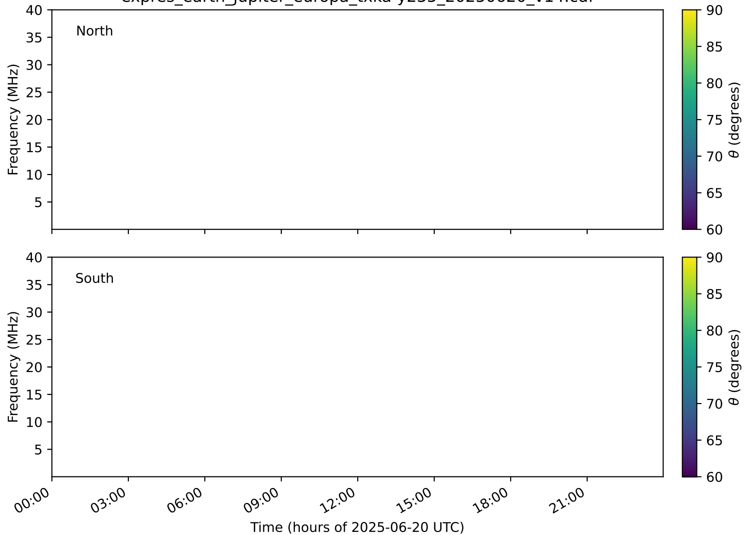
expres_earth_jupiter_europa_txka-y235_20250620_v14.cdf
