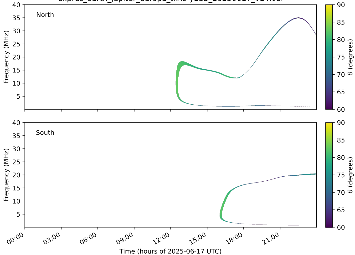
expres_earth_jupiter_europa_txka-y235_20250617_v14.cdf
