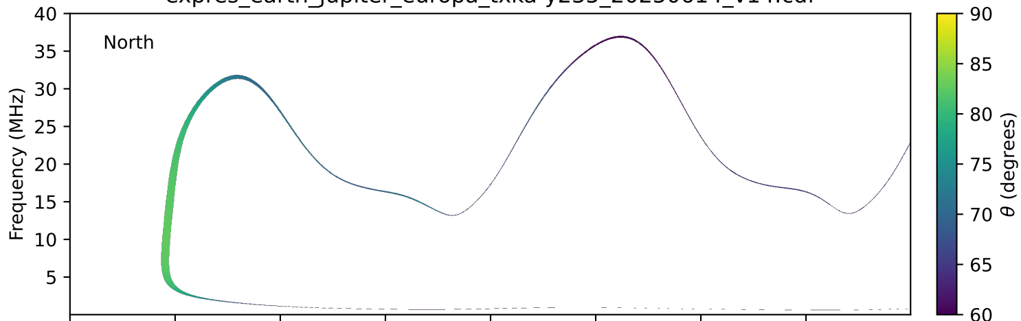
expres_earth_jupiter_europa_txka-y235_20250614_v14.cdf
