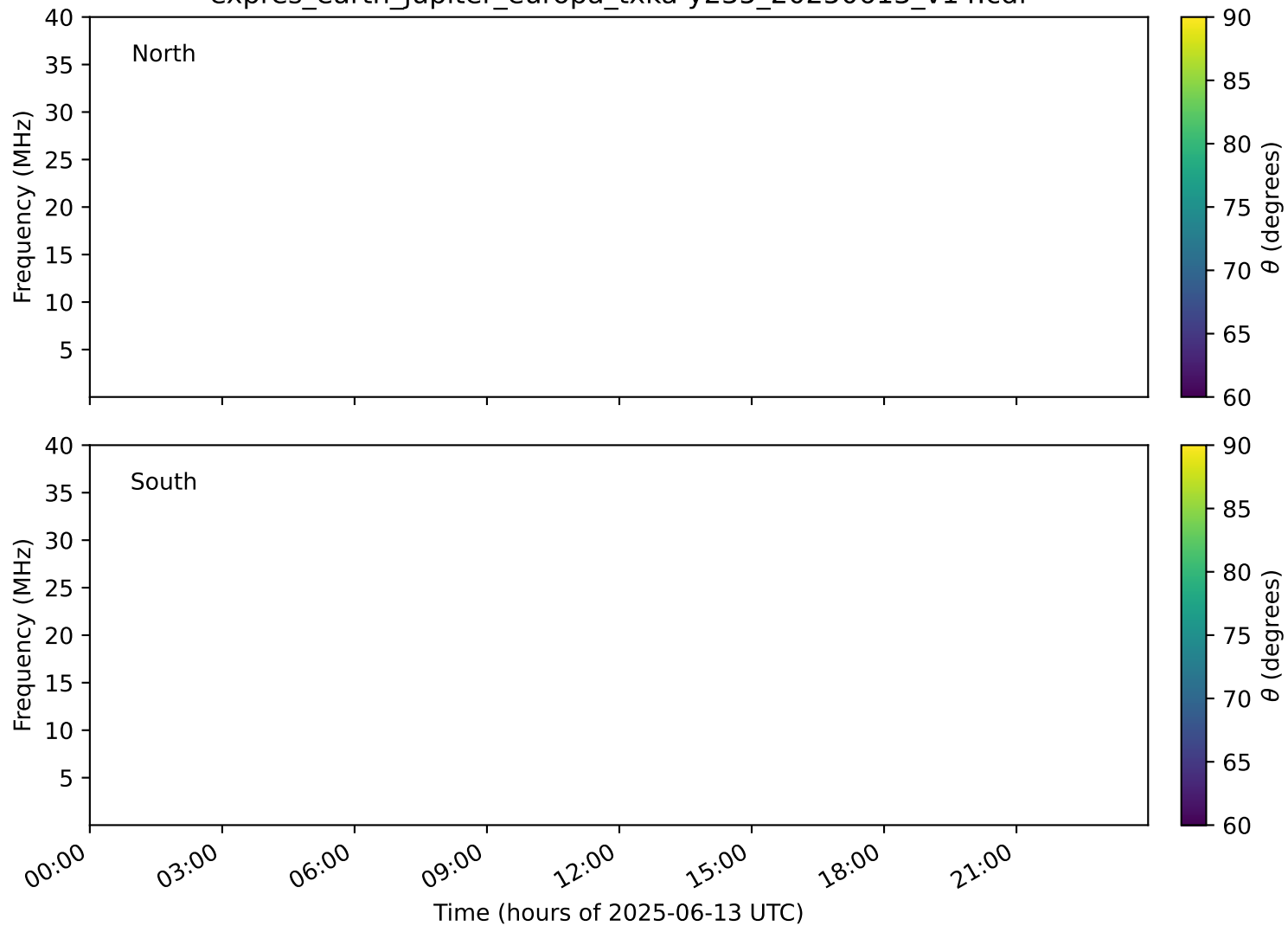
expres_earth_jupiter_europa_txka-y235_20250613_v14.cdf
