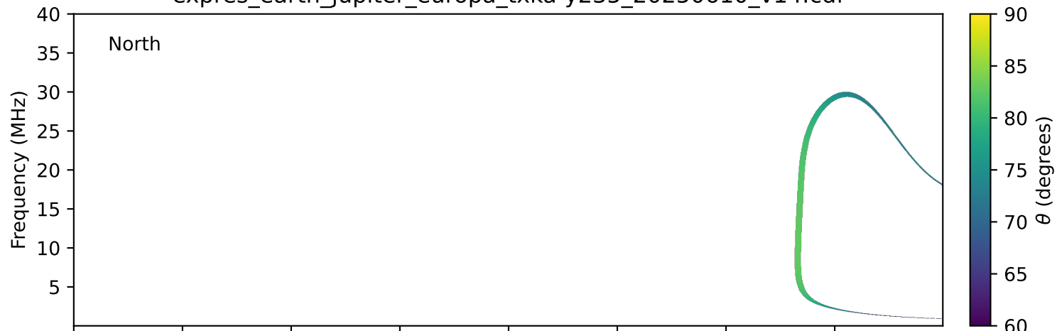
expres_earth_jupiter_europa_txka-y235_20250610_v14.cdf
