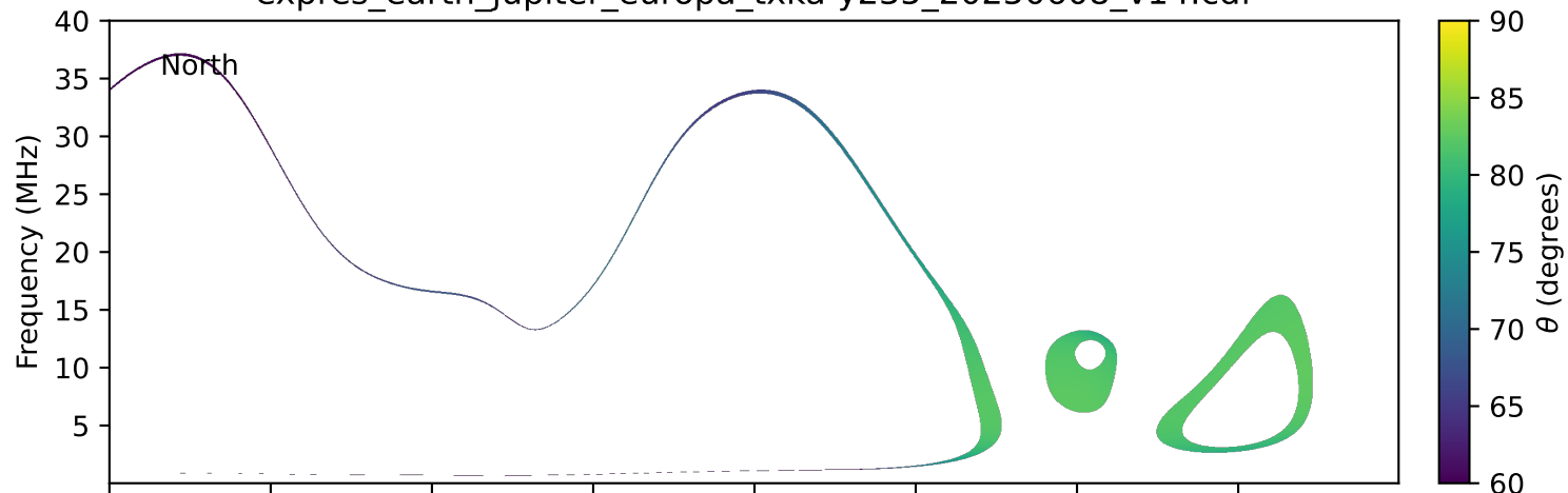
expres_earth_jupiter_europa_txka-y235_20250608_v14.cdf
