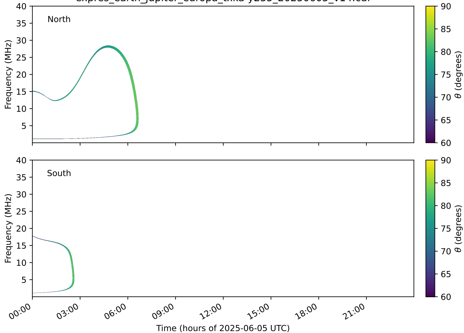
expres_earth_jupiter_europa_txka-y235_20250605_v14.cdf
