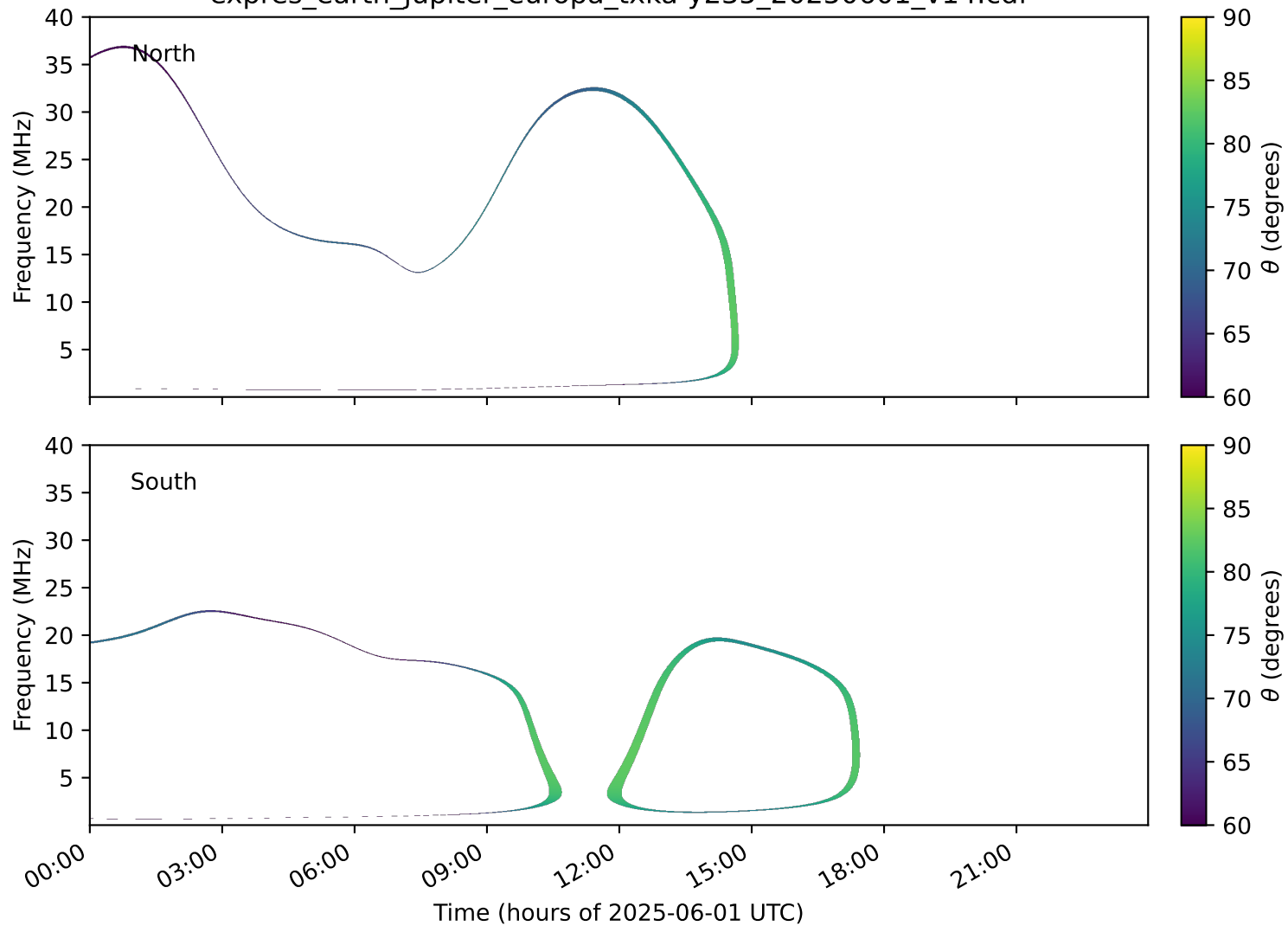
expres_earth_jupiter_europa_txka-y235_20250601_v14.cdf
