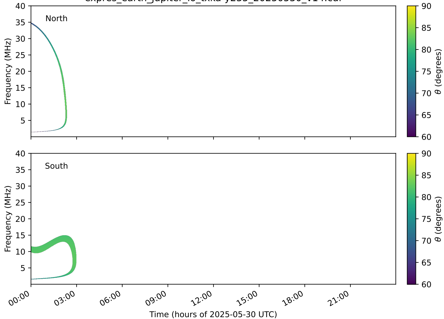
expres_earth_jupiter_io_txka-y235_20250530_v14.cdf
