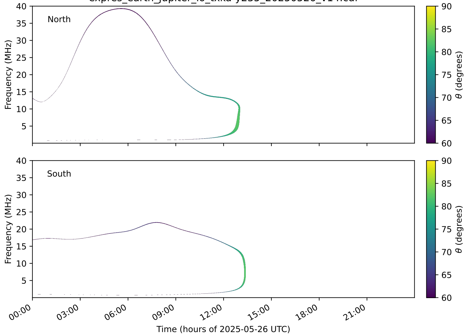
expres_earth_jupiter_io_txka-y235_20250526_v14.cdf
