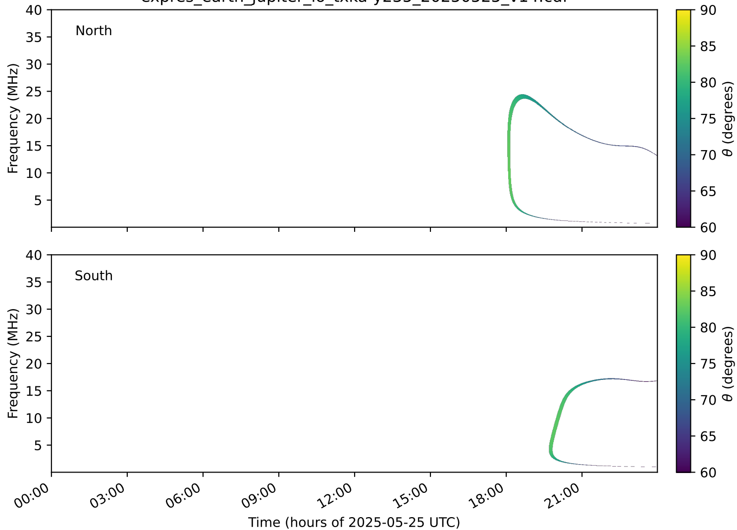
expres_earth_jupiter_io_txka-y235_20250525_v14.cdf
