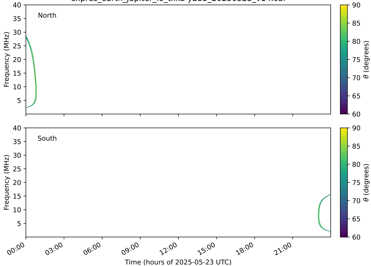
expres_earth_jupiter_io_txka-y235_20250523_v14.cdf
