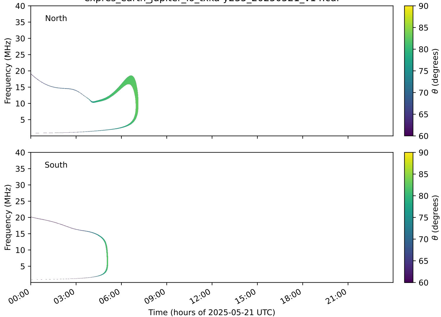
expres_earth_jupiter_io_txka-y235_20250521_v14.cdf
