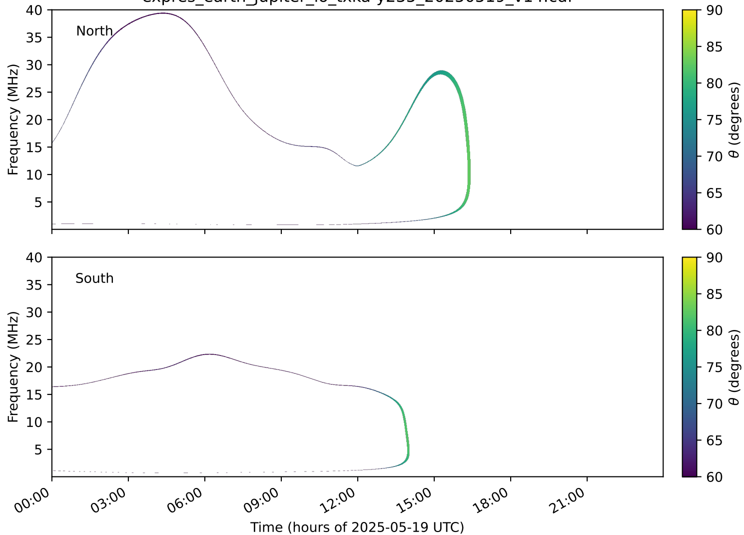
expres_earth_jupiter_io_txka-y235_20250519_v14.cdf
