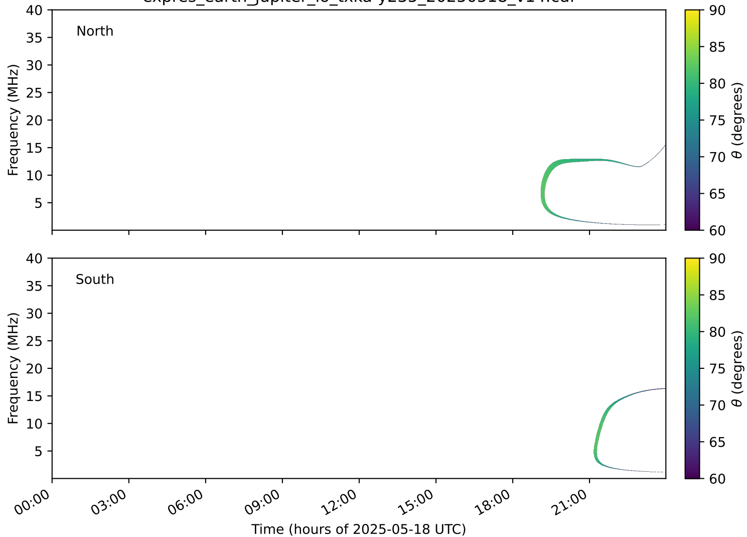
expres_earth_jupiter_io_txka-y235_20250518_v14.cdf
