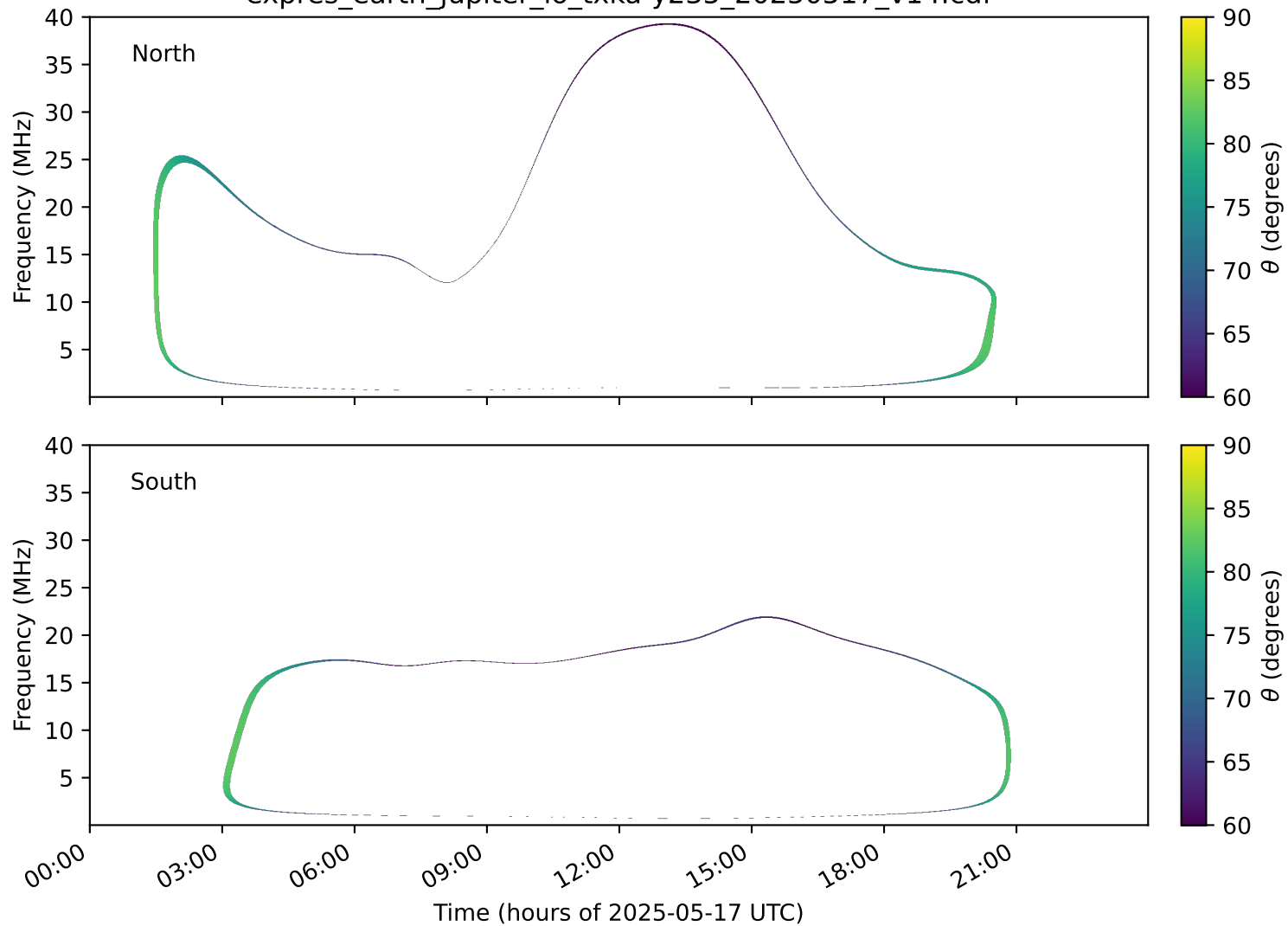
expres_earth_jupiter_io_txka-y235_20250517_v14.cdf
