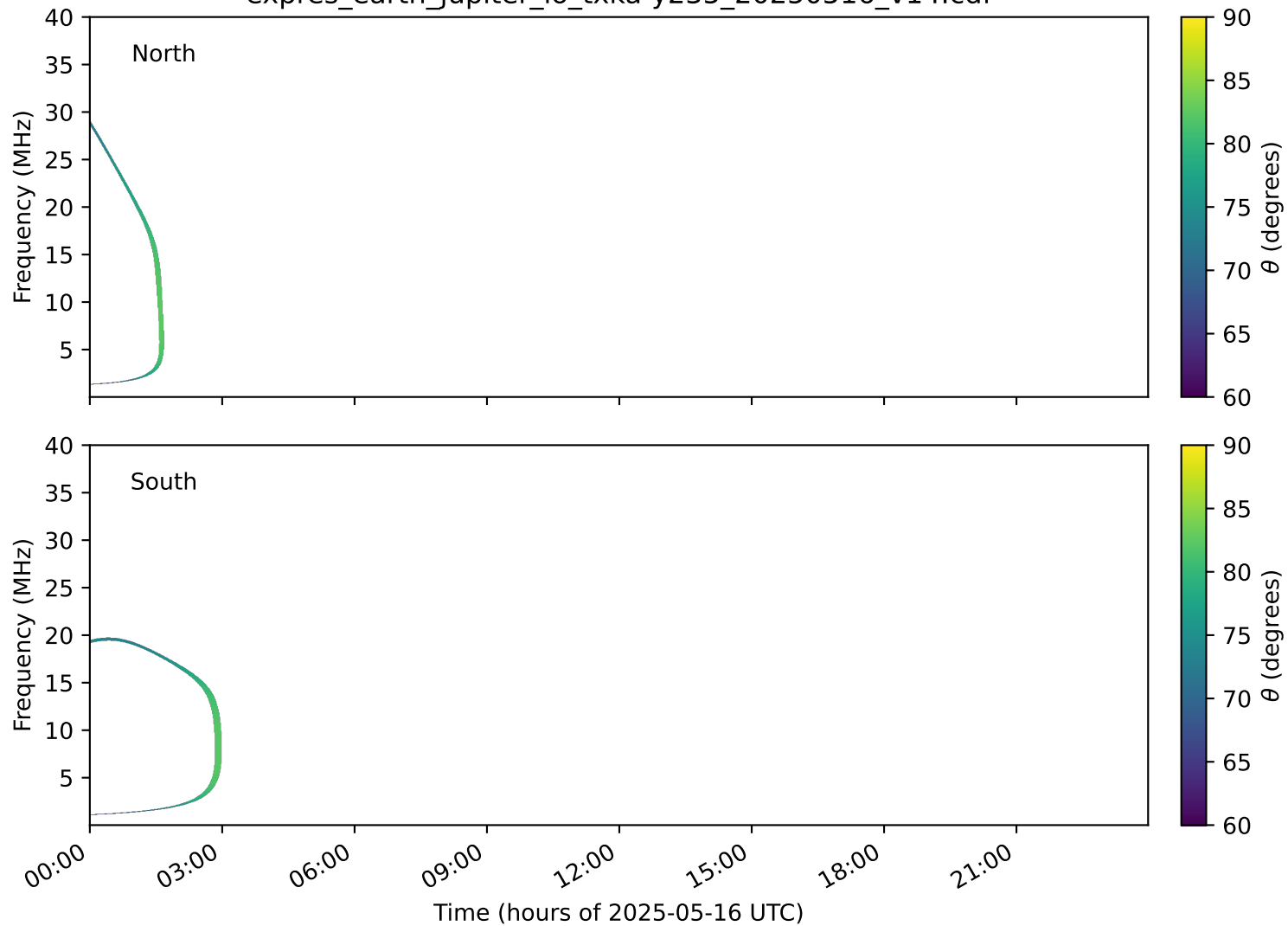
expres_earth_jupiter_io_txka-y235_20250516_v14.cdf
