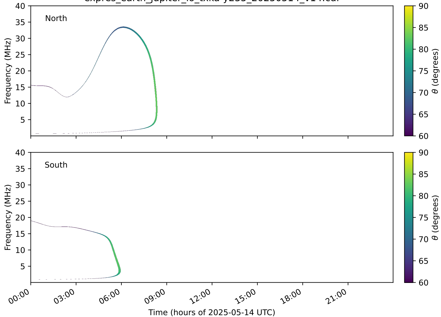
expres_earth_jupiter_io_txka-y235_20250514_v14.cdf
