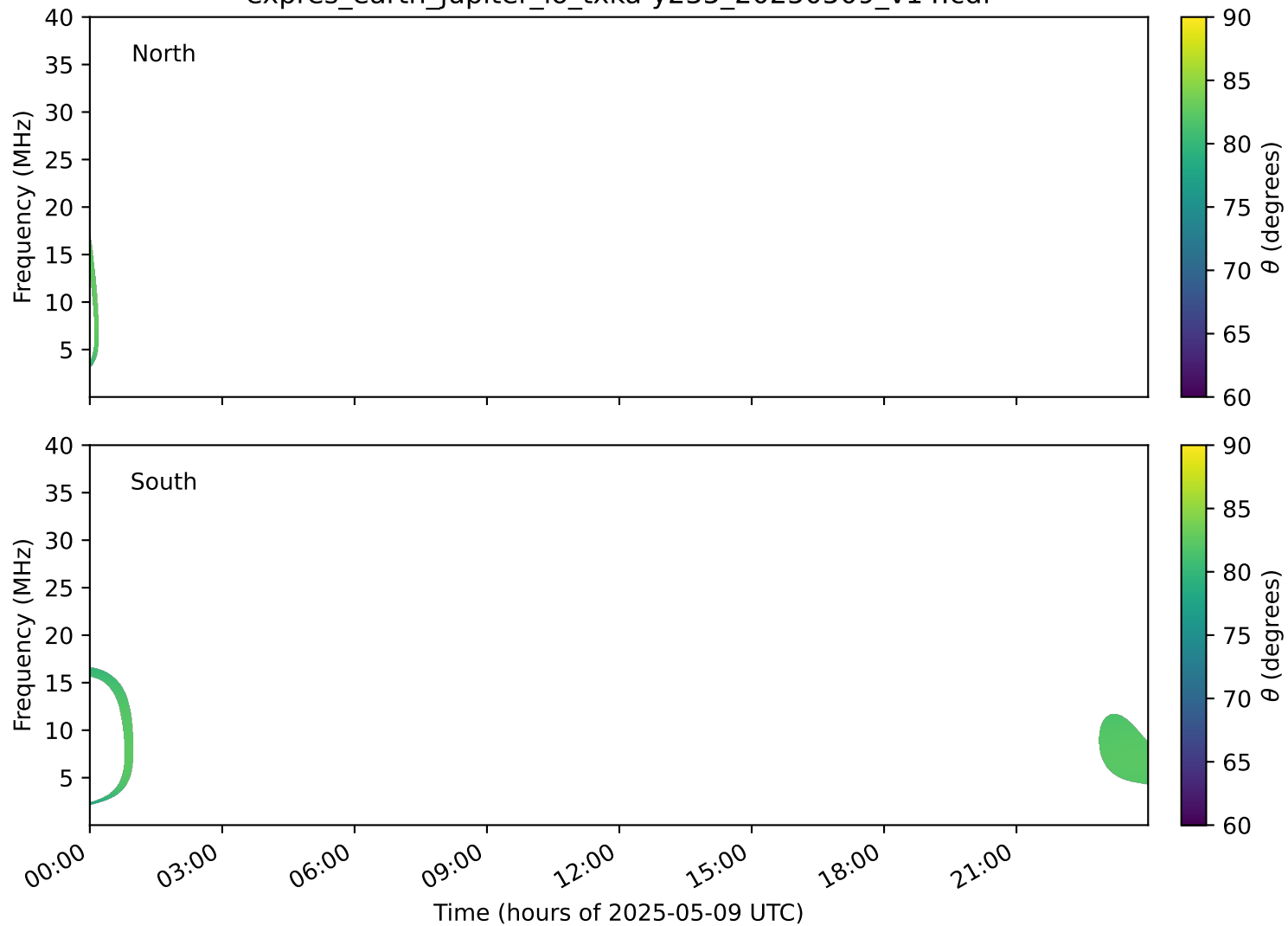
expres_earth_jupiter_io_txka-y235_20250509_v14.cdf
