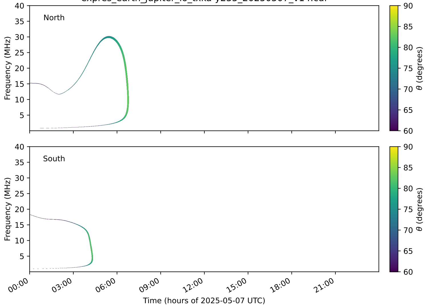
expres_earth_jupiter_io_txka-y235_20250507_v14.cdf
