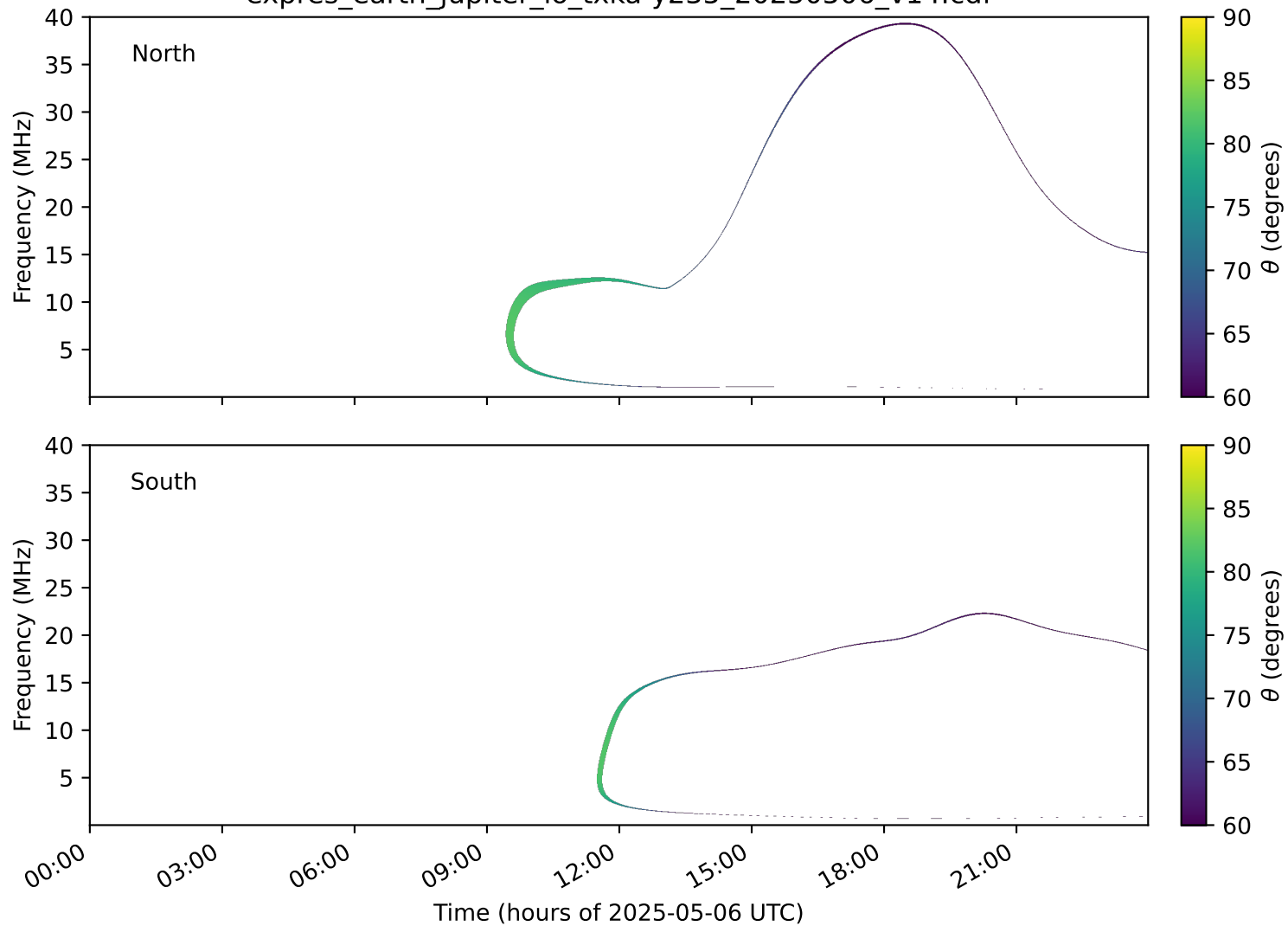
expres_earth_jupiter_io_txka-y235_20250506_v14.cdf
