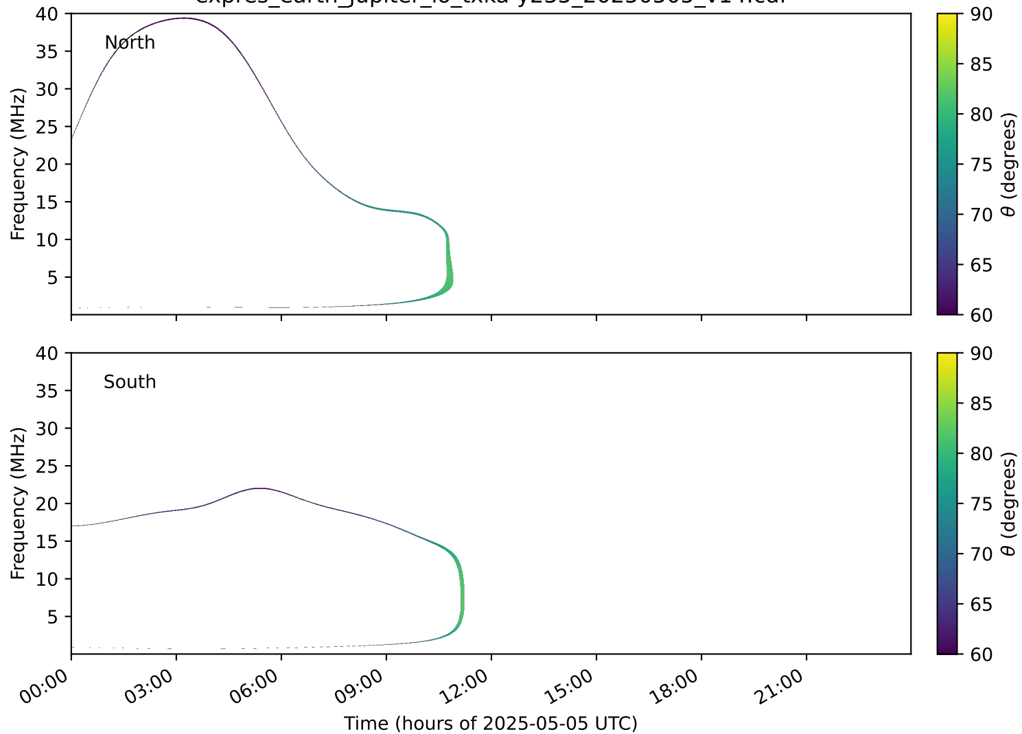
expres_earth_jupiter_io_txka-y235_20250505_v14.cdf
