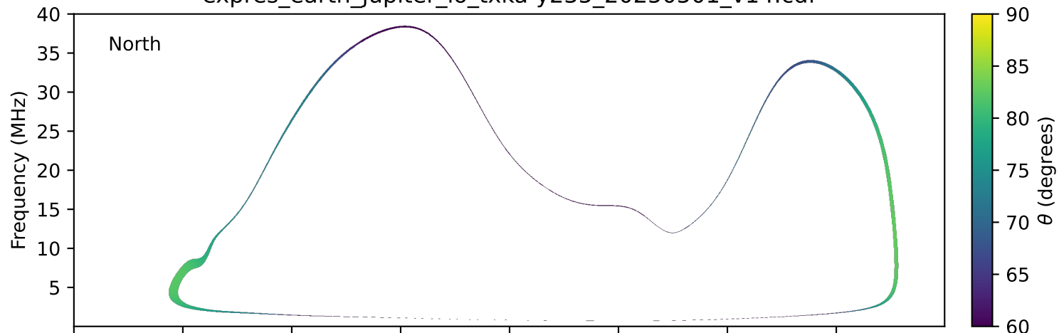
expres_earth_jupiter_io_txka-y235_20250501_v14.cdf
