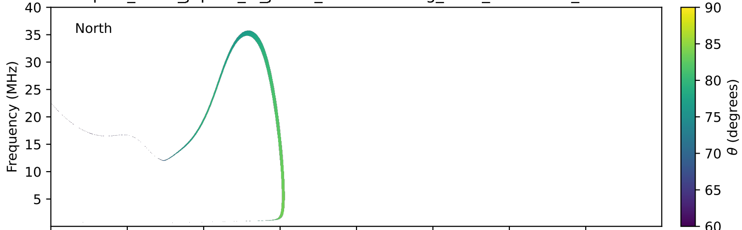
expres_earth_jupiter_io_jrm33_lossc-wid1deg_3kev_20250528_v11.cdf
