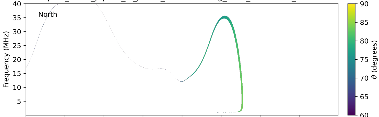
expres_earth_jupiter_io_jrm33_lossc-wid1deg_3kev_20250519_v11.cdf
