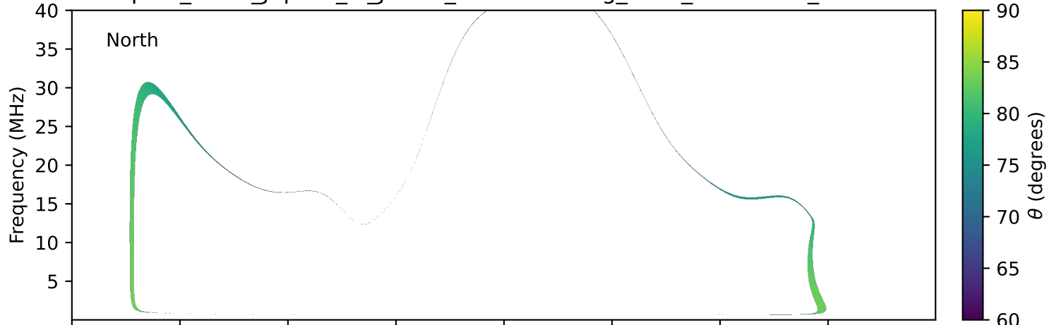
expres_earth_jupiter_io_jrm33_lossc-wid1deg_3kev_20250517_v11.cdf
