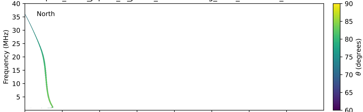
expres_earth_jupiter_io_jrm33_lossc-wid1deg_3kev_20250516_v11.cdf
