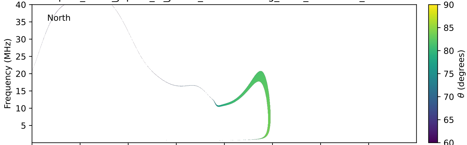
expres_earth_jupiter_io_jrm33_lossc-wid1deg_3kev_20250512_v11.cdf
