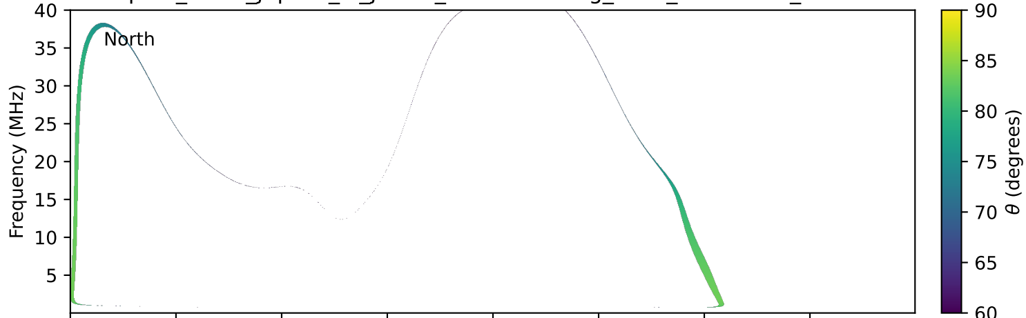
expres_earth_jupiter_io_jrm33_lossc-wid1deg_3kev_20250510_v11.cdf
