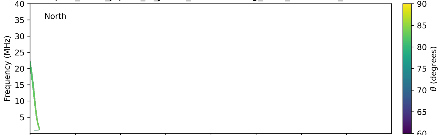
expres_earth_jupiter_io_jrm33_lossc-wid1deg_3kev_20250509_v11.cdf
