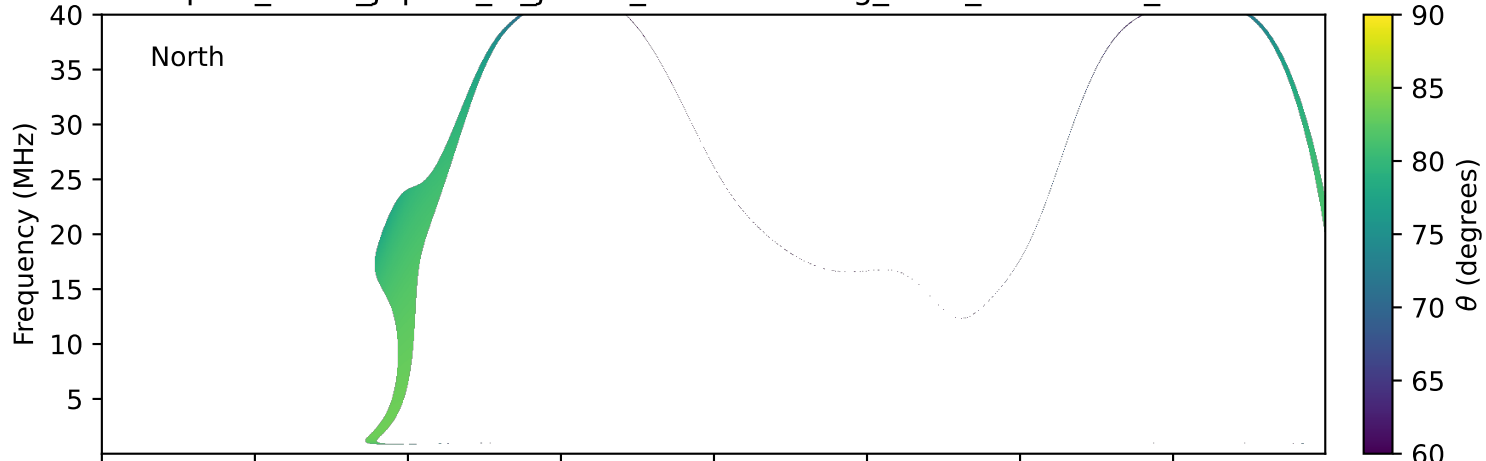
expres_earth_jupiter_io_jrm33_lossc-wid1deg_3kev_20250508_v11.cdf
