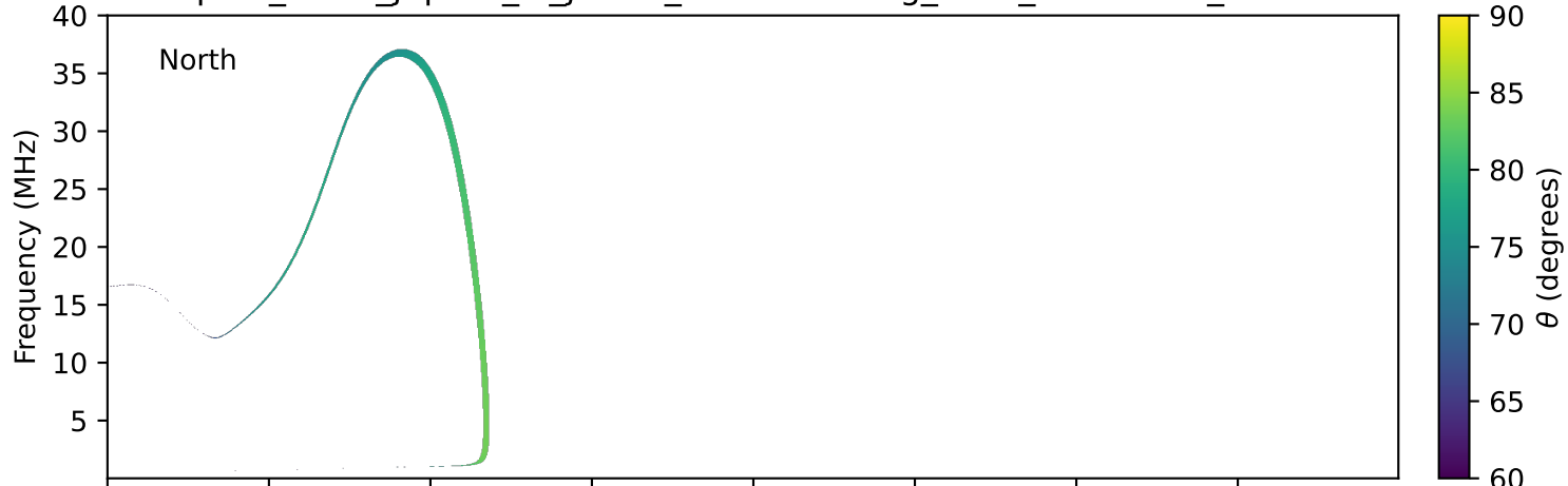
expres_earth_jupiter_io_jrm33_lossc-wid1deg_3kev_20250507_v11.cdf
