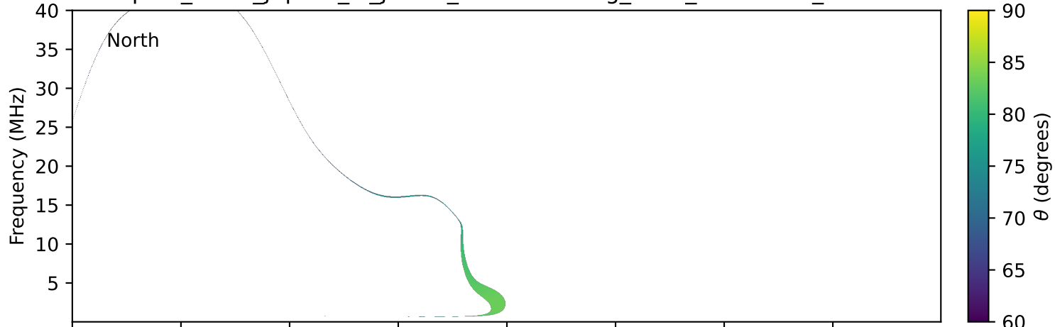
expres_earth_jupiter_io_jrm33_lossc-wid1deg_3kev_20250505_v11.cdf
