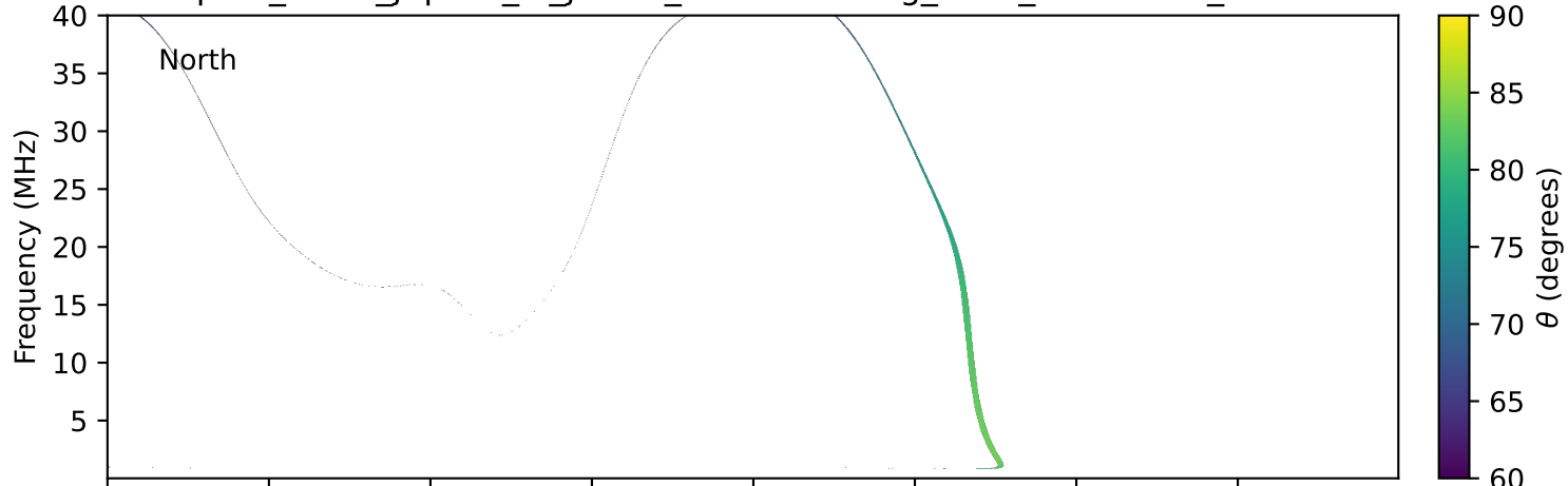
expres_earth_jupiter_io_jrm33_lossc-wid1deg_3kev_20250503_v11.cdf
