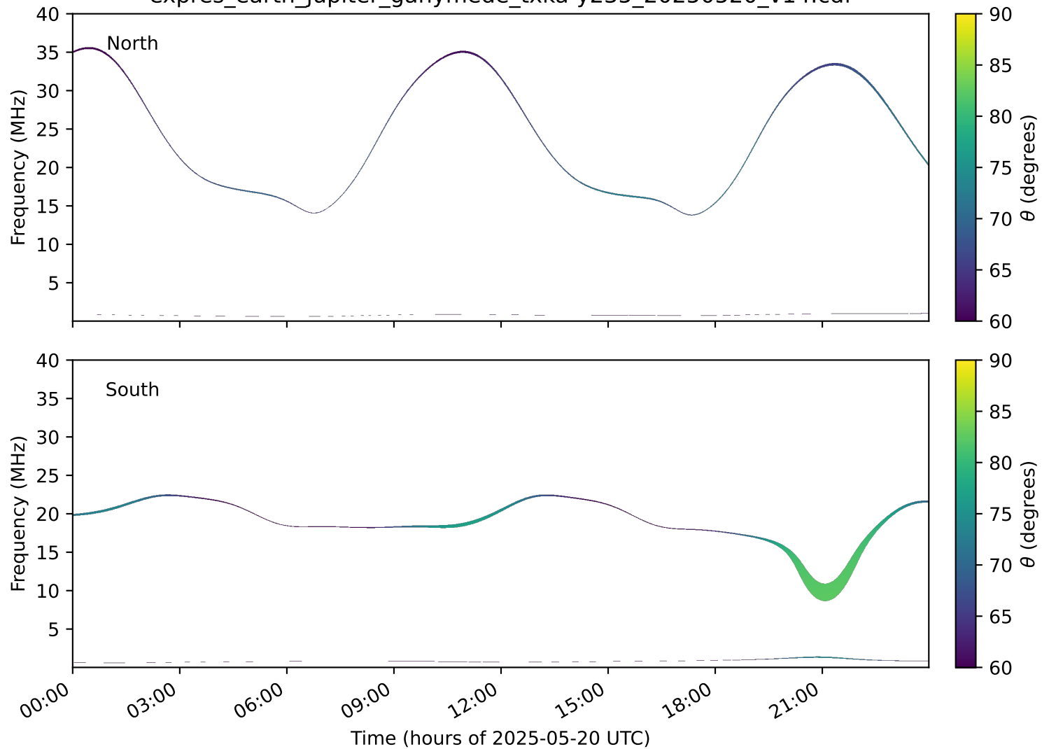
expres_earth_jupiter_ganymede_txka-y235_20250520_v14.cdf
