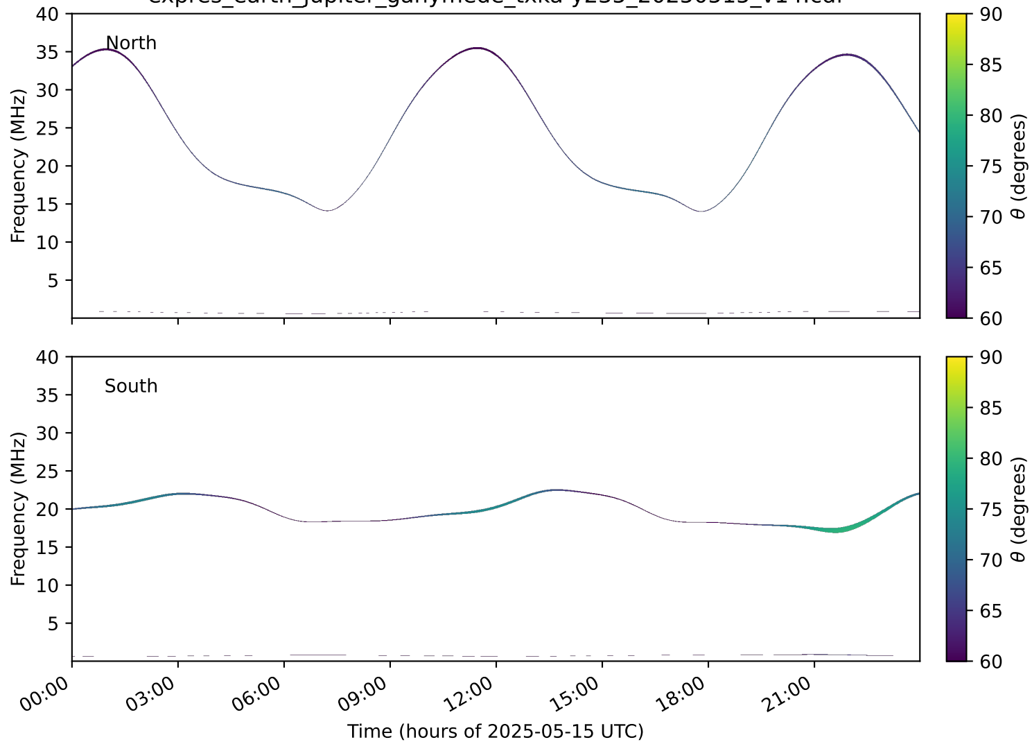
expres_earth_jupiter_ganymede_txka-y235_20250515_v14.cdf
