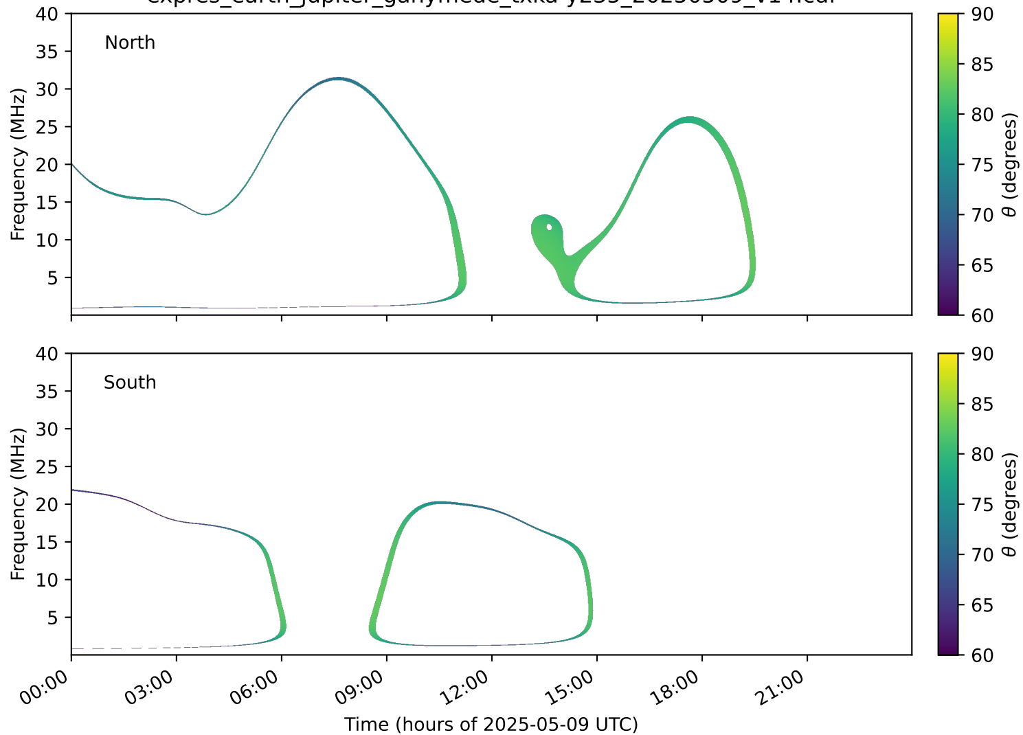
expres_earth_jupiter_ganymede_txka-y235_20250509_v14.cdf
