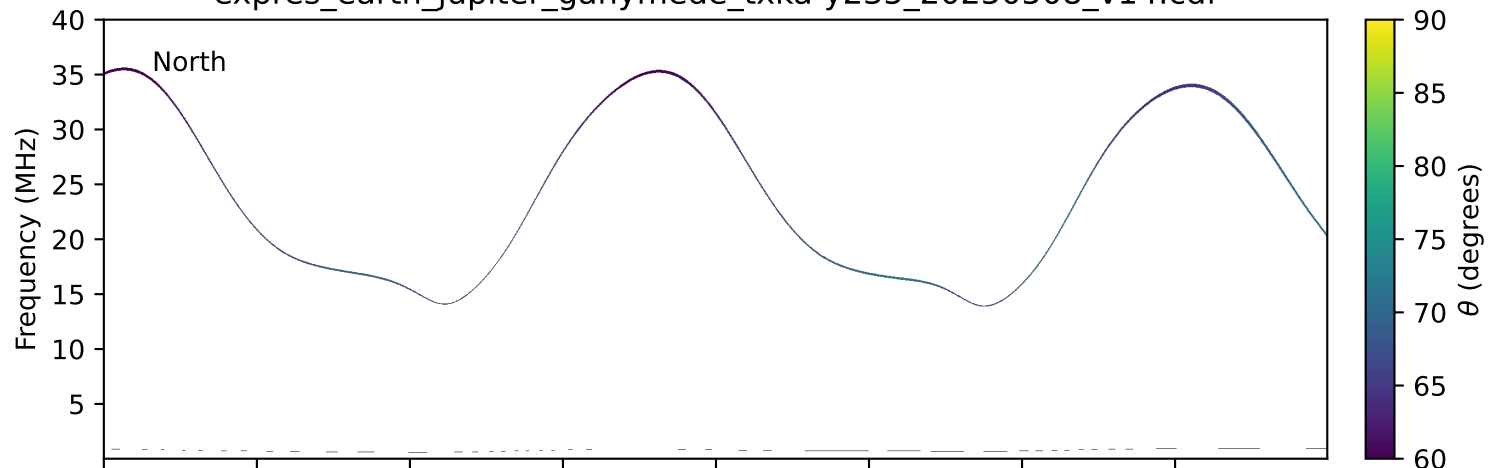
expres_earth_jupiter_ganymede_txka-y235_20250508_v14.cdf
