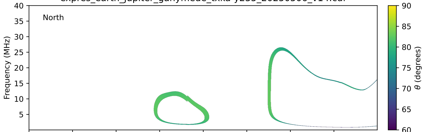
expres_earth_jupiter_ganymede_txka-y235_20250506_v14.cdf
