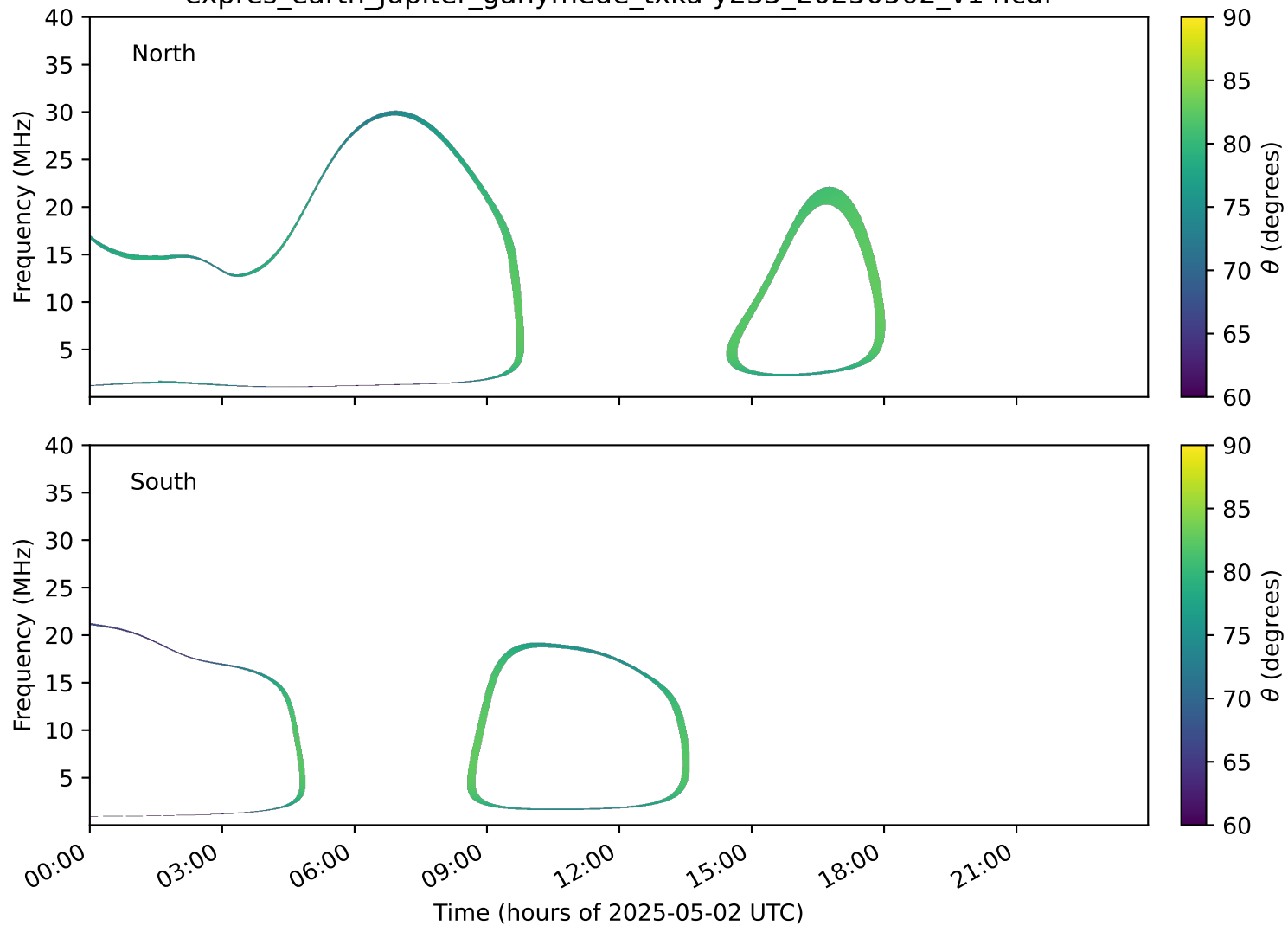
expres_earth_jupiter_ganymede_txka-y235_20250502_v14.cdf
