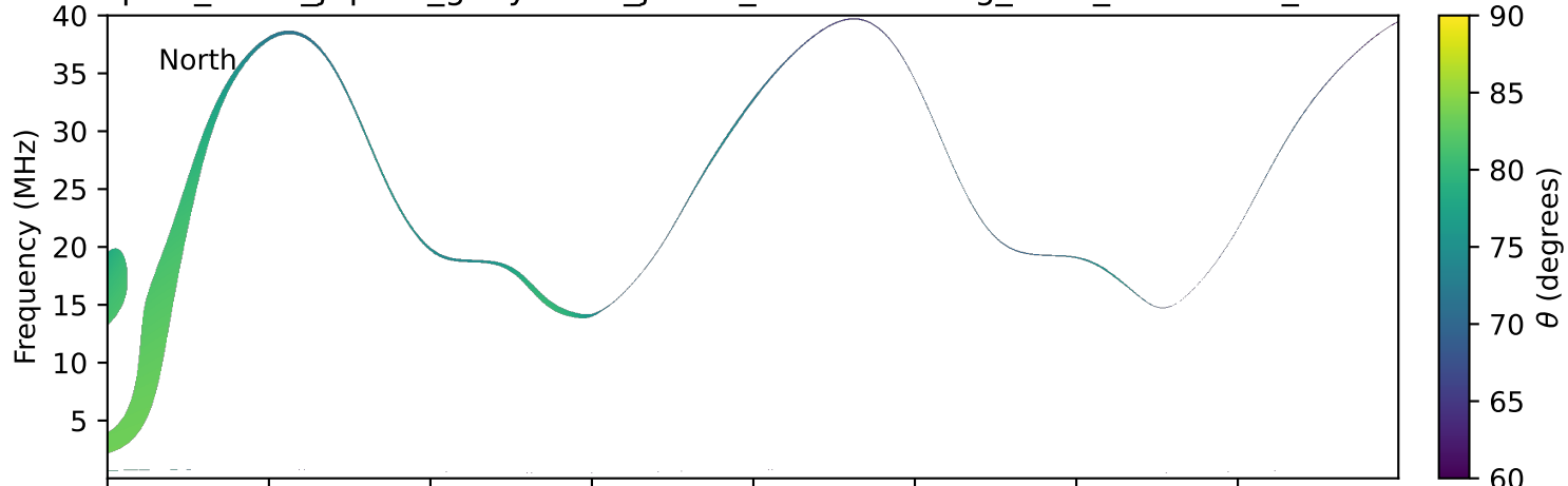
expres_earth_jupiter_ganymede_jrm33_lossc-wid1deg_3kev_20250507_v11.cdf
