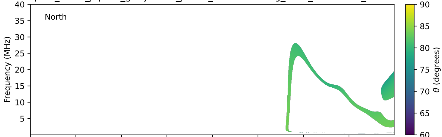
expres_earth_jupiter_ganymede_jrm33_lossc-wid1deg_3kev_20250506_v11.cdf
