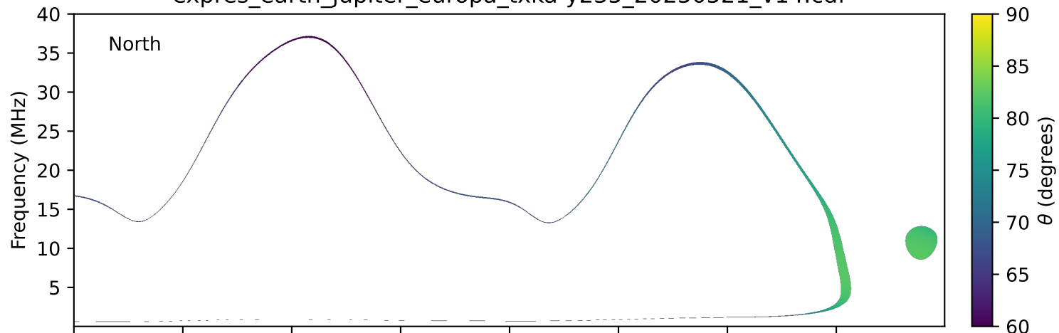
expres_earth_jupiter_europa_txka-y235_20250521_v14.cdf
