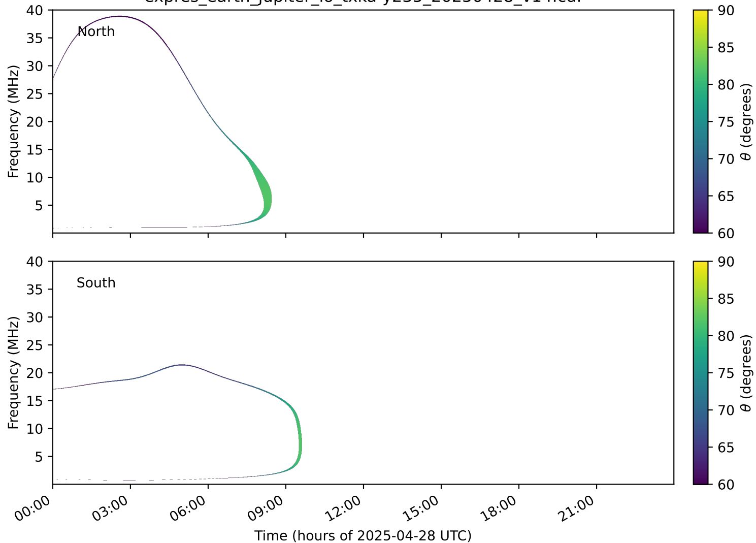
expres_earth_jupiter_io_txka-y235_20250428_v14.cdf
