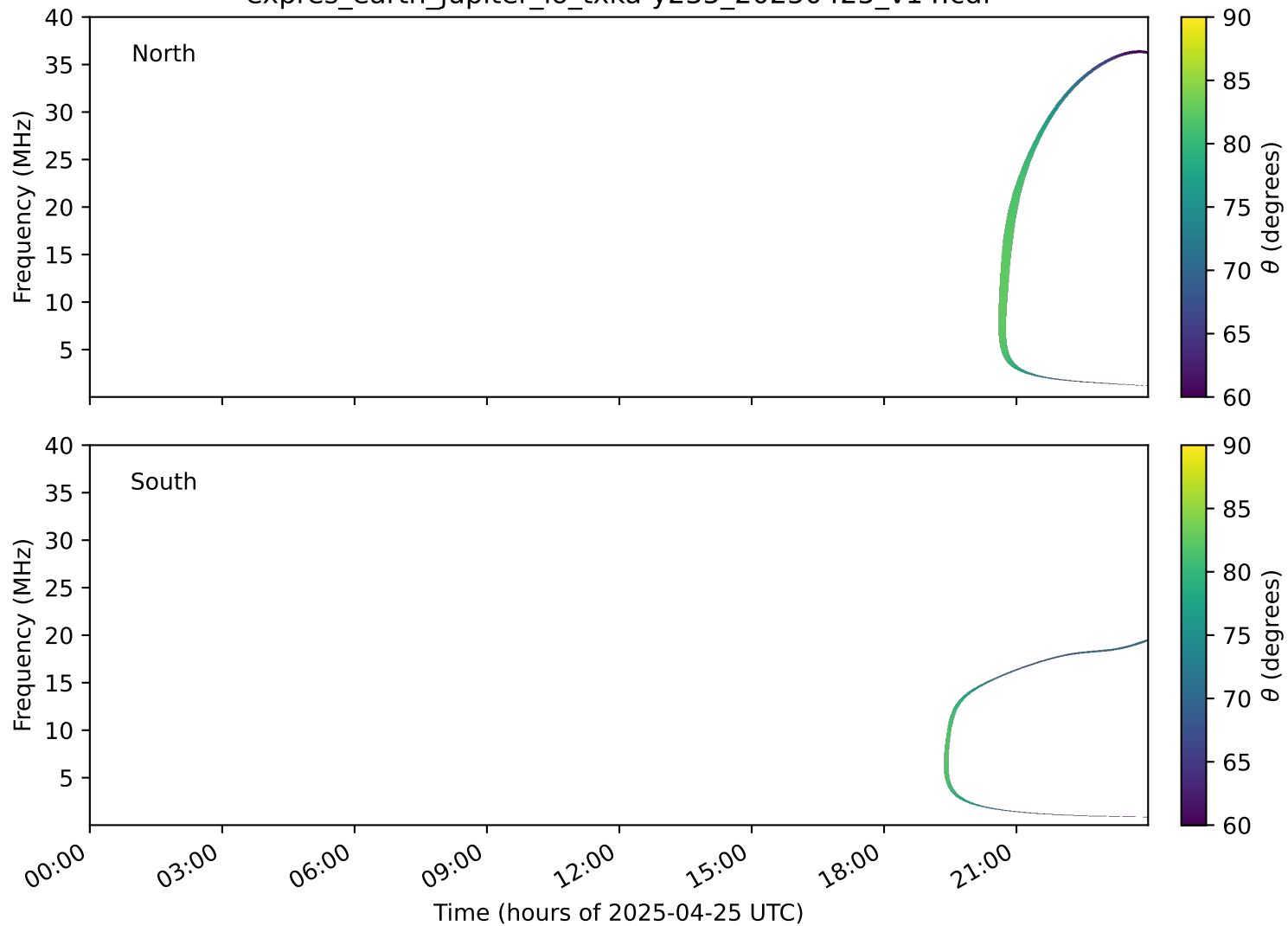
expres_earth_jupiter_io_txka-y235_20250425_v14.cdf
