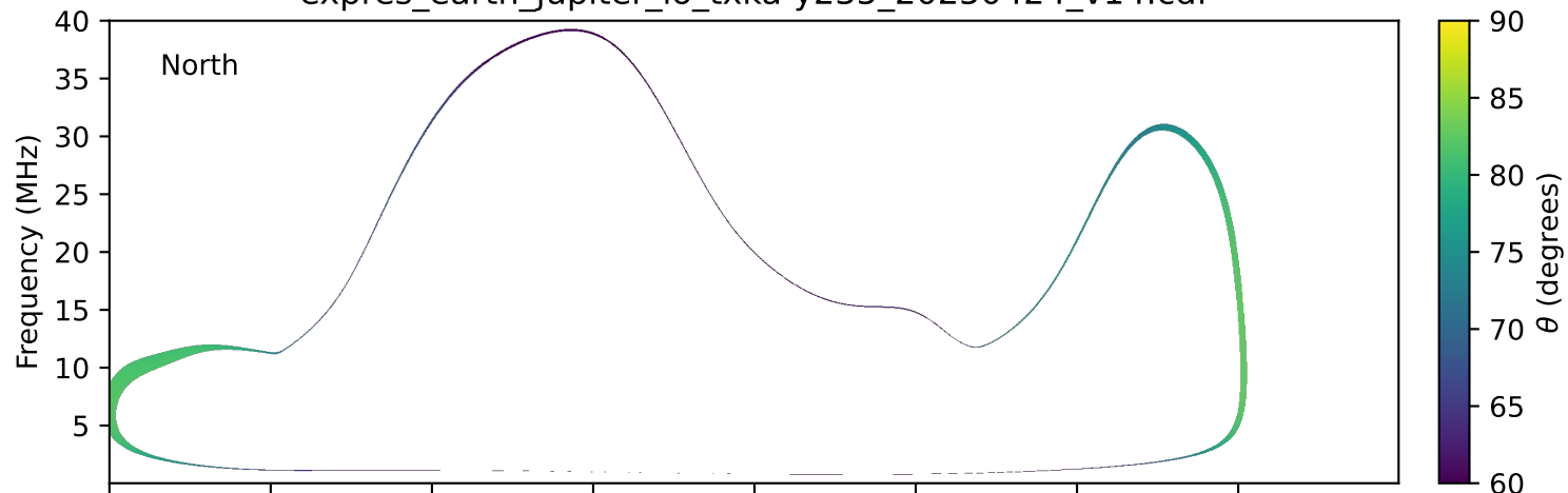
expres_earth_jupiter_io_txka-y235_20250424_v14.cdf
