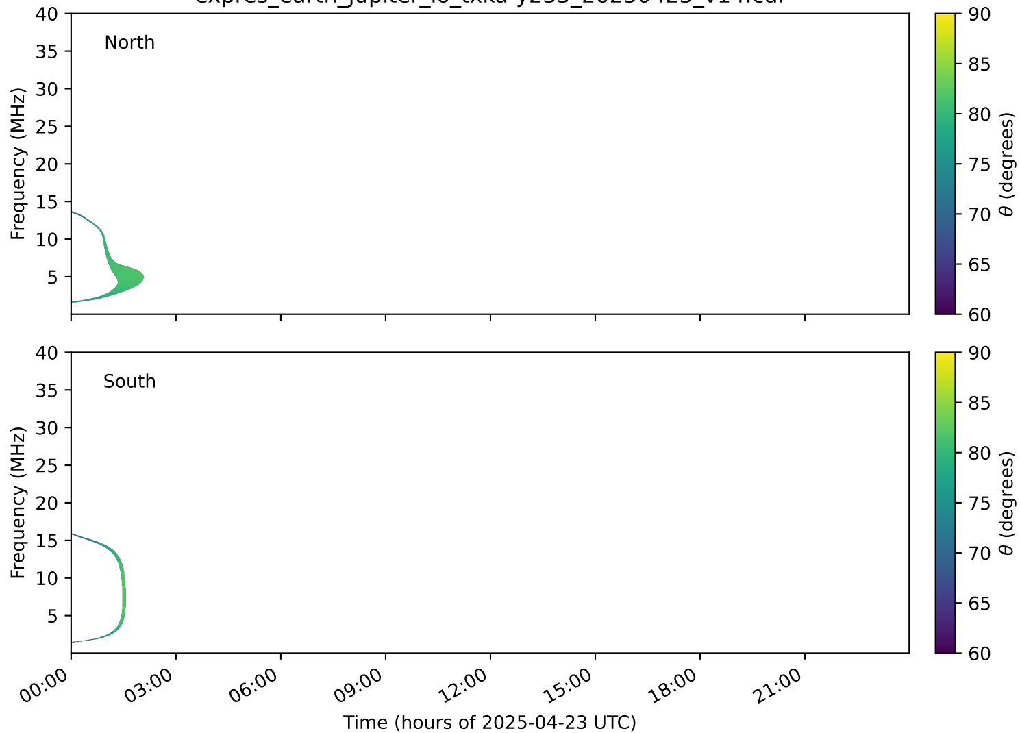
expres_earth_jupiter_io_txka-y235_20250423_v14.cdf
